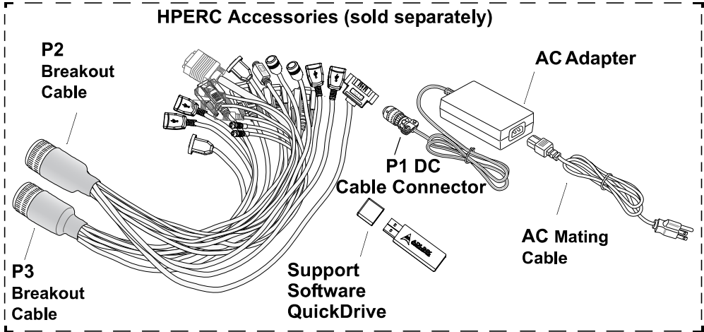
Figure 1-1: HPERC Unit with Accessories
