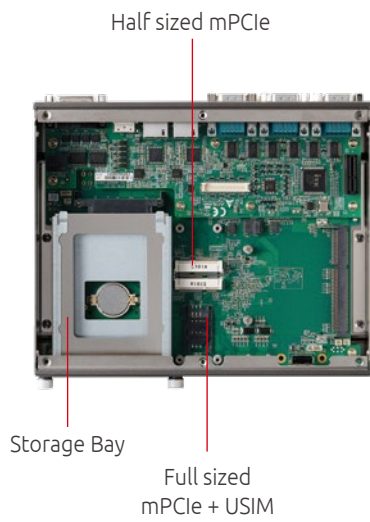
Rich I/O Enables Seamless Interconnection
