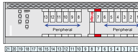
cPCIS-2633R/cPCIS-2833R Inside Rear View
