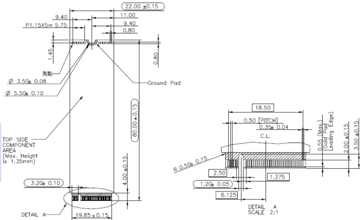
Top View
